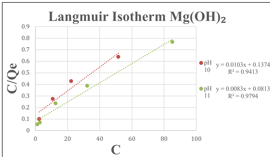
Figure 23: Langmuir Isotherm results for Mg(OH)_2 .
