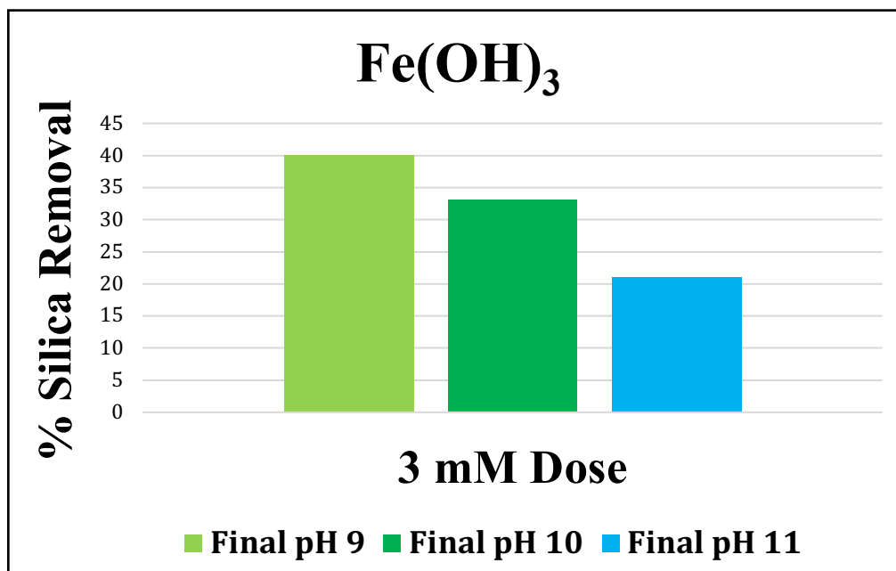
Figure 19: The Percent Silica Removal vs. pH at a 3 mM Dose of \text{Fe}(\text{OH})_3 .
