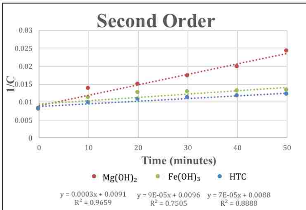
Figure 32: Second Order Kinetic results.
