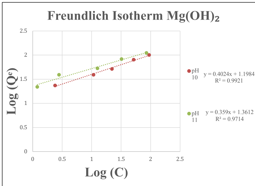
Figure 22: Freundlich Isotherm results for Mg(OH)_2 .
